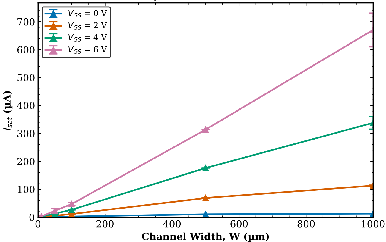
TFT1 Combined (Tr. 1 & 2) I_{sat} vs W | L = 8\text{ }\mu\text{m} (mean \pm std)
